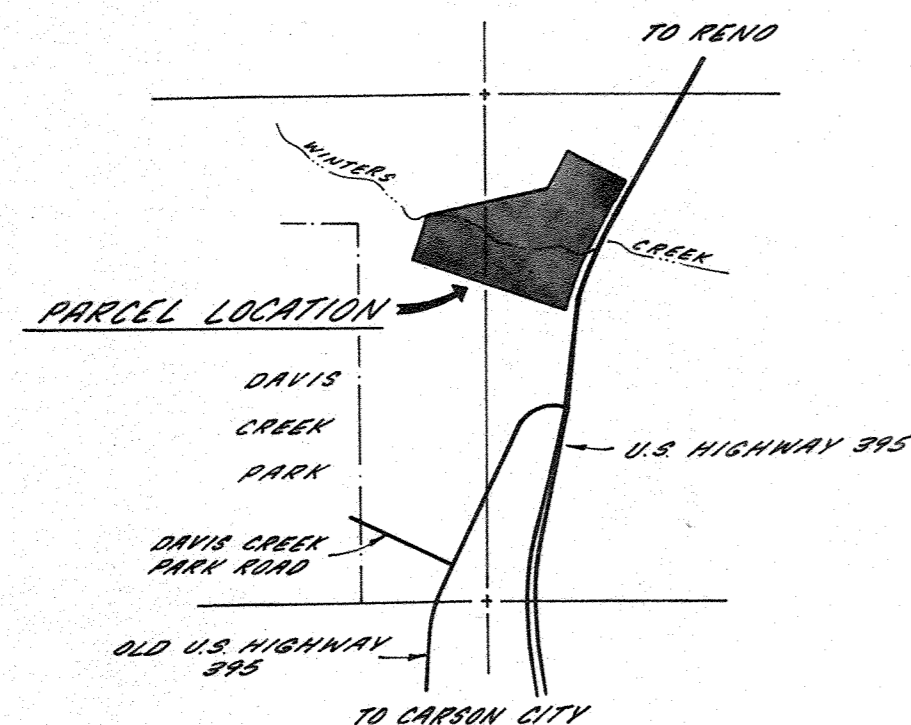
SECTIONS 26 & 27, T.17N., R.19E., M.D.B. & M. VICINITY MAP SCALE: 1" = 200'
